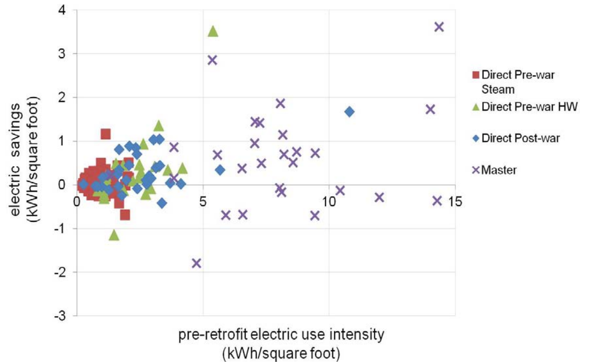
Figure 10: Electric Savings by Comparative Group vs. Pre-retrofit Electric Use Intensity
