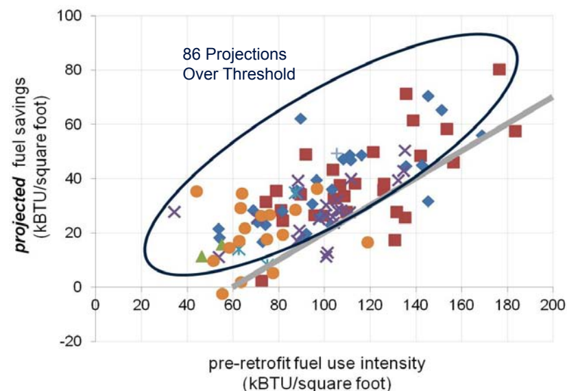
Using the Threshold To Determine More Conservative Projections Projected Fuel Savings vs. Pre-retrofit Fuel Use Intensity
