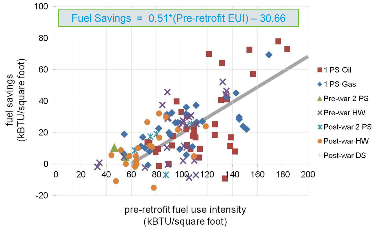
Figure 12: Relationship Between Buildings' Actual Post-retrofit Savings and Pre-retrofit Fuel Consumption Actual Fuel Savings vs. Pre-retrofit Fuel Use Intensity
