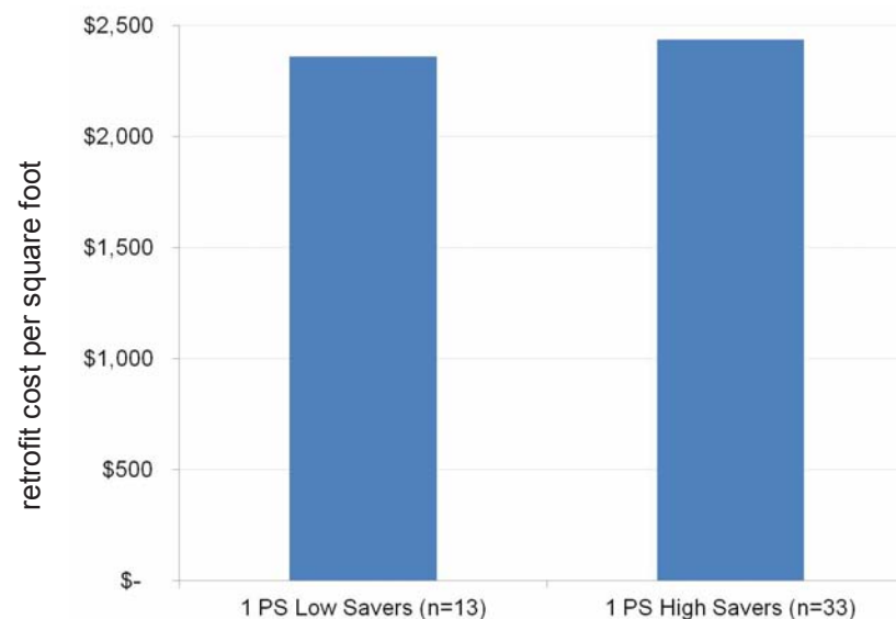
Figure 26: One-pipe Steam High Savers vs. Low Savers, Fuel Measures
